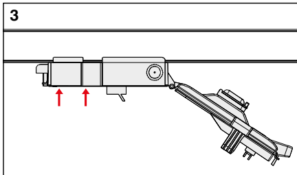
3- Carefully align the tap off box contacts and push the box towards the busbar.
