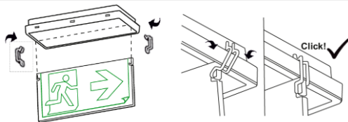
EXIT TRNO Two-Sided Flag 250x124x3mm
